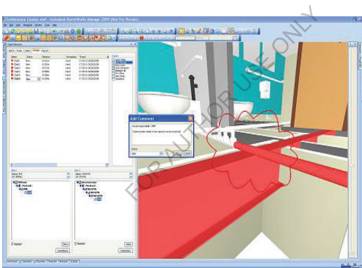
Figure 3. An example of identifying the interactions of structural and mechanical models and specifying it by the BIM management team
